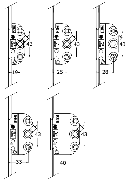
DORN / BACKSET 19, 25, 28, 33, 40 MM
